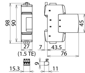
Dimension drawing DG SE CI 440 FM
