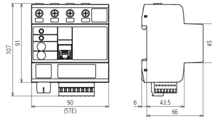
Dimension drawing DRC SD 1 1
