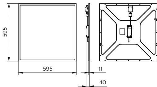
RC132V G4 LED43S/840 PSU W60L60 NOC
