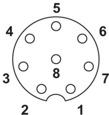
Pin assignment
