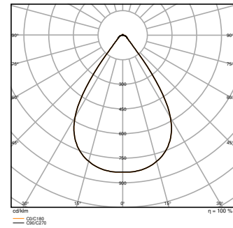
HB P 125W 840 70DEG IP66 PS
