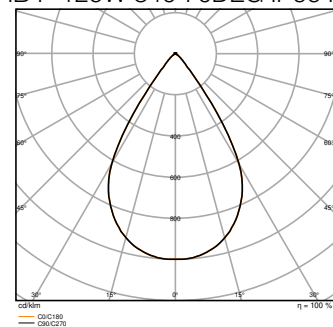
HB P 150W 840 70DEG IP66 PS - REFLECTOR
