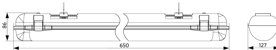
LEDWaterproof-CLA-E L650
