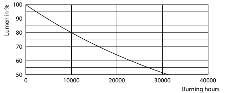
Lumen Maintenance Diagram - LEDbulb ND 13-100W A67 E27 827 2CT
