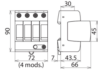
Dimension drawing DG MU 3PY 600 4W+G
