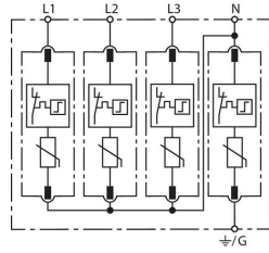
Basic circuit diagram DG MU 3PY 600 4W+G
