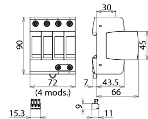
Dimension drawing DG M TNS 385 FM
