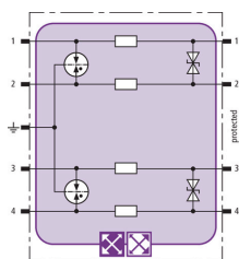
Basic circuit diagram BXT ML4 BD 12
