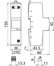
Dimension drawing DGPM 1 255 FM
