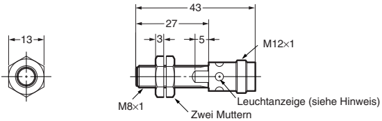
E2A-S08KS02-M1-□□
