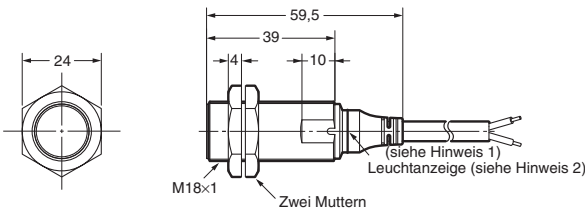
E2A-M18KS08-WP-□□/E2A-S18KS08-WP-□
