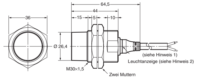
E2A-M30KN20-WP-□□/E2A-S30KN20-WP-□
