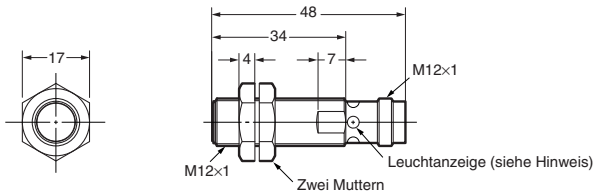
E2A-M12KS04-M1-□□/E2A-S12KS04-M1-□
