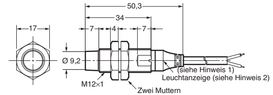
E2A-M12KN08-WP-□□/E2A-S12KN08-WP-□
