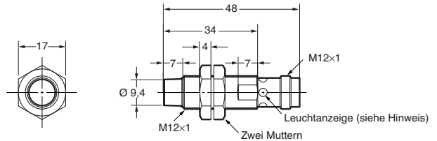
E2A-M12KN08-M1-□□/E2A-S12KN08-M1-□
