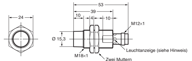
E2A-M18KN16-M1-□□/E2A-S18KN16-M1-□
