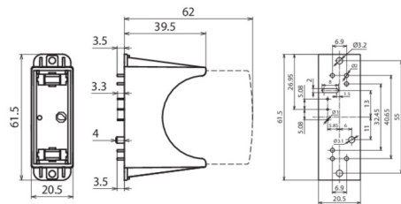
Dimension drawing DG PCB PV I 600 FM
