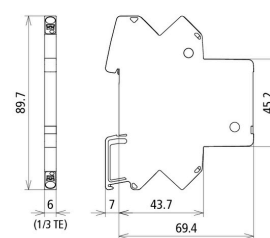
Dimension drawing BCO CL2 BE 48
