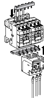
LAD9VP2 = LAD9V10 + LAD9V6
