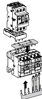
LAD9VP1 = LAD9V5 + LAD9V11
