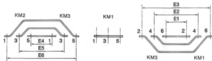
Power links dimensions for 3 identical contactors
