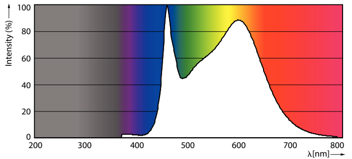
Spectral Power Distribution Colour - CorePro LEDBulbND10.5-100W E27A60 840CLG
