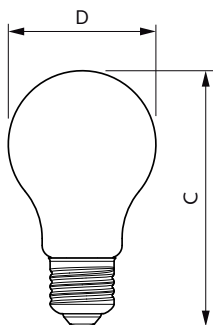
MASTER VLE LEDBulbD7.2-50W E27 A60 827 CM G
