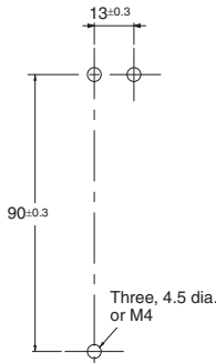
Mounting Holes
