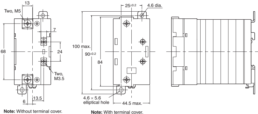
Mounting Holes
