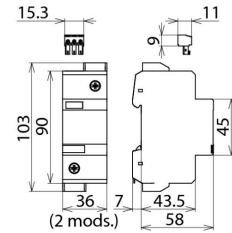
Dimension drawing DG 1000 FM
