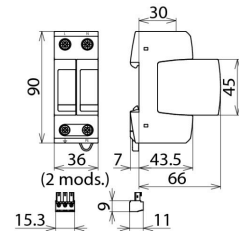
Dimension drawing DG M TT 2P 320 FM
