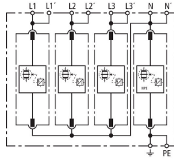
Basic circuit diagram DV M TT 255
