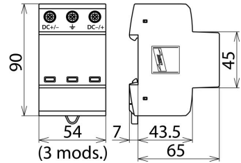
Dimension drawing DG YPV SCI 600
