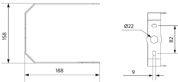
LEDHighbay-P5 Bracket-D330
