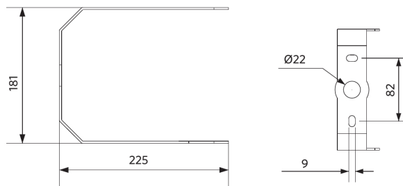
LEDHighbay-P5 Bracket-D420
