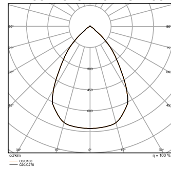
HB P 75W 840 110DEG IP66 PS - REFLECTOR
