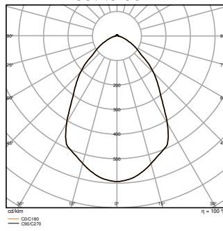
HB P 75W 840 110DEG IP66 PS - REFRACTOR
