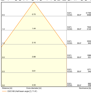
HB P 75W 840 110DEG IP66 PS - REFLECTOR
