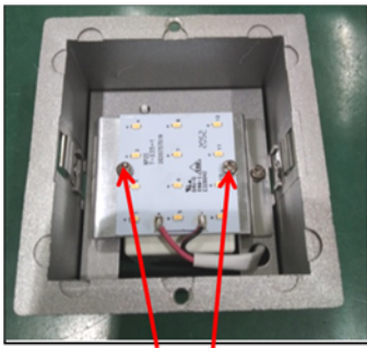
Figure 4 Remove the screws
