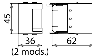
Dimension drawing DSE MOD 220
