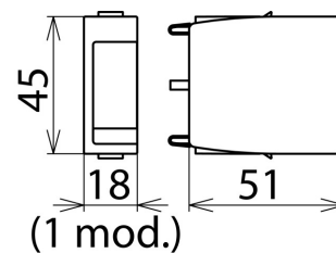
Dimension drawing DG PLU 180
