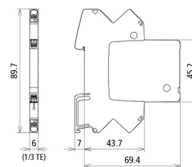
Dimension drawing BCO ML2 BD 48
