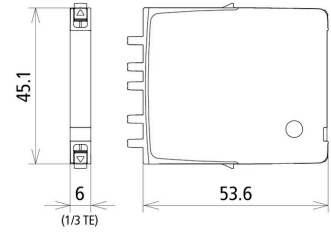
Dimension drawing BCO MOD ML2 BPD 24
