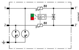
Basic circuit diagram BCO MOD ML2 BPD 24
