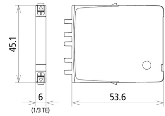
Dimension drawing BCO MOD ML2 BD HF 5
