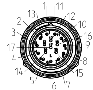
socket face female
