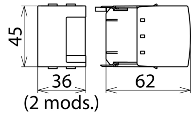
Dimension drawing DSE MOD 60
