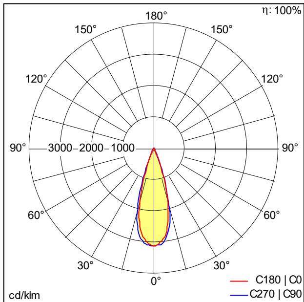
TE_LILY_LED_SPOT_IP44_24_68_850_930.idt
