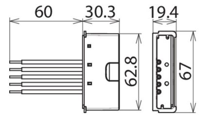
Dimension drawing DCOR L 3P 275 SO LTG
