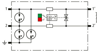
Basic circuit diagram BCO MOD ML2 EX 24
