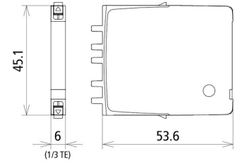
Dimension drawing BCO MOD ML2 EX 24
